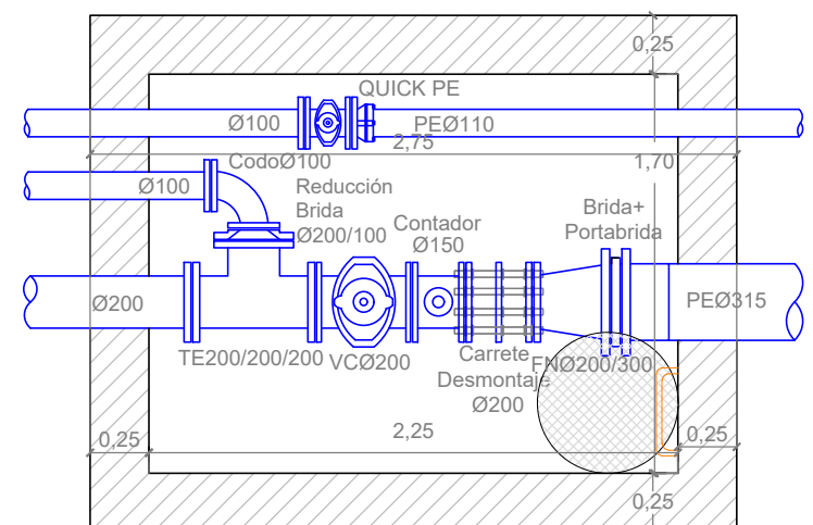
Nudo Manantial (NM)_Planta
