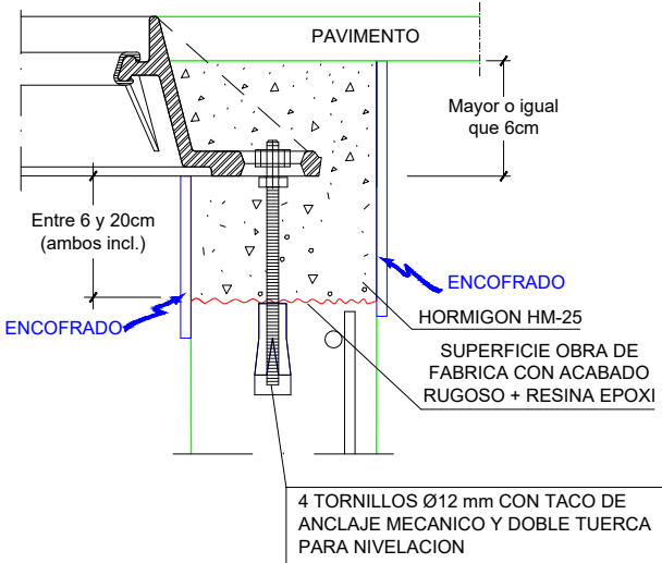
DETALLE 1. E=1/5
