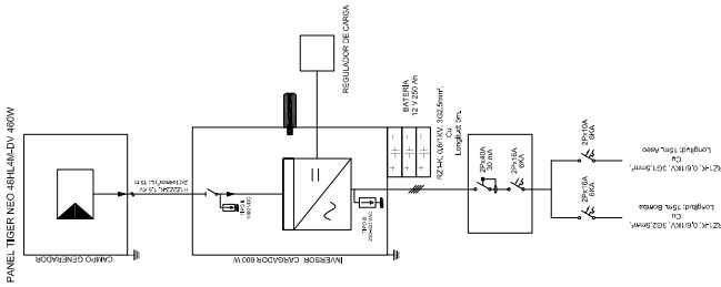
UNIFILAR INSTALACION ELECTRICA
