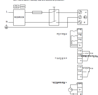
Example of mains-connected motor with main switch, backup fuse and additional protection
