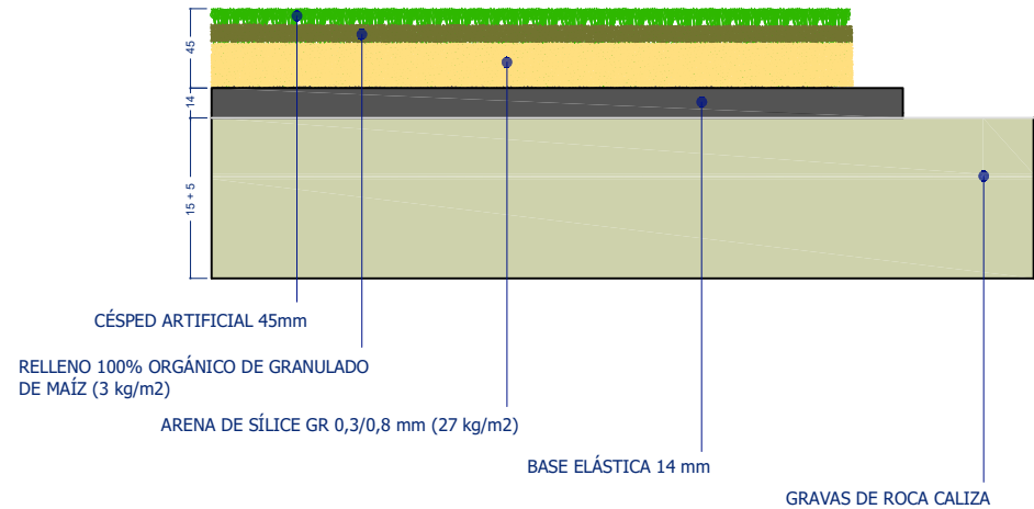
DETALLE CÉSPED ARTIFICIAL
