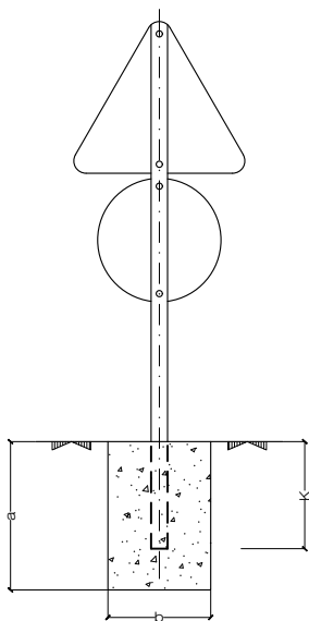
DOS SENALES TRIANGULAR - CIRCULAR
