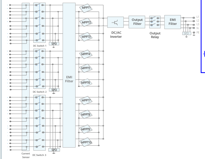
Circuit Diagram
