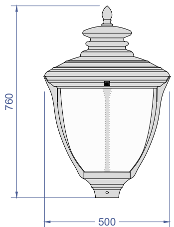
LUMINARIA SELENE
