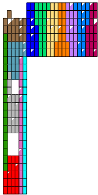
Inversor 1
