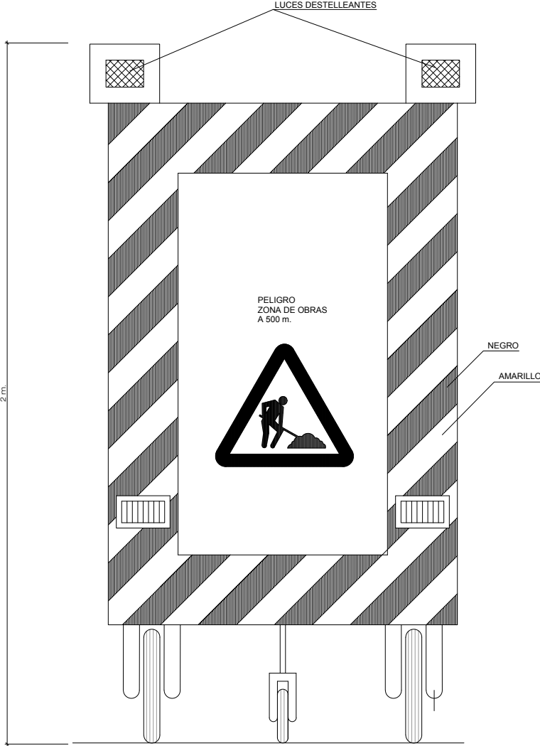
VISTA FRONTAL
