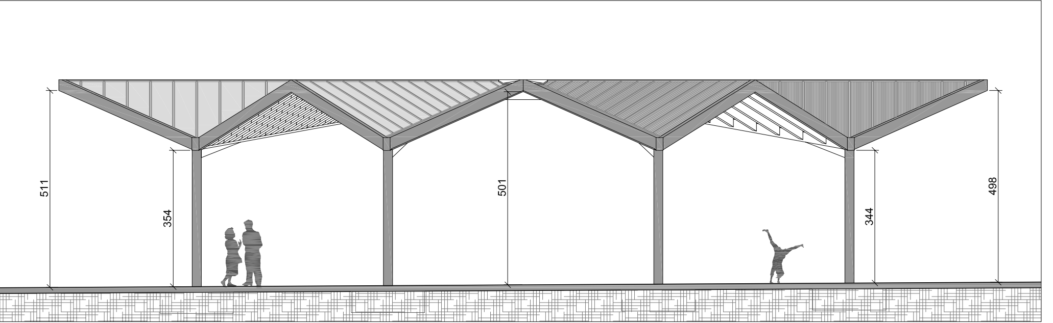
ALZADO DIAGONAL
