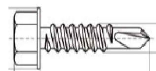
H-DIN 7504 K 6,3x75mm Autotaladrante
