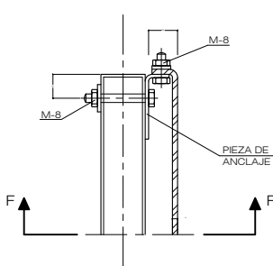
DETALLE -E-
