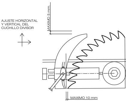
CUCHILLO DIVISOR
